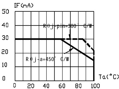
FIG.5 MAXIMUM FORWARD DC CURRENT VS TEMPERATURE. DERATING BASED ON T_{jmax}=125^{\circ}\text{C}
